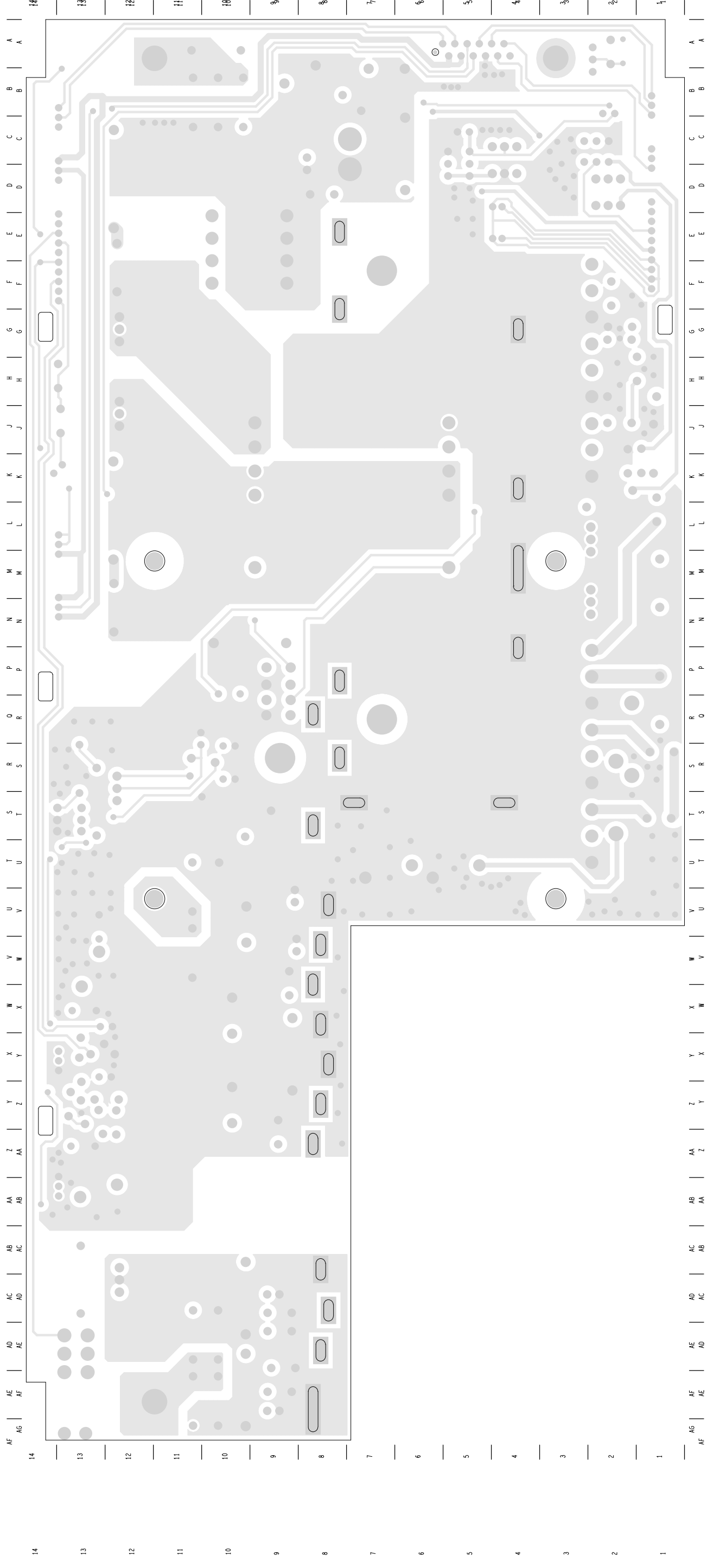
TAIT ELECTRONICS 220-02041-03 A 30Mg/05 NTS TB8000 24V DC-DC CONVERTER LAYOUT-SECONDARY-SIDE
